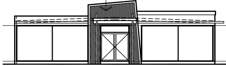
east elevation
