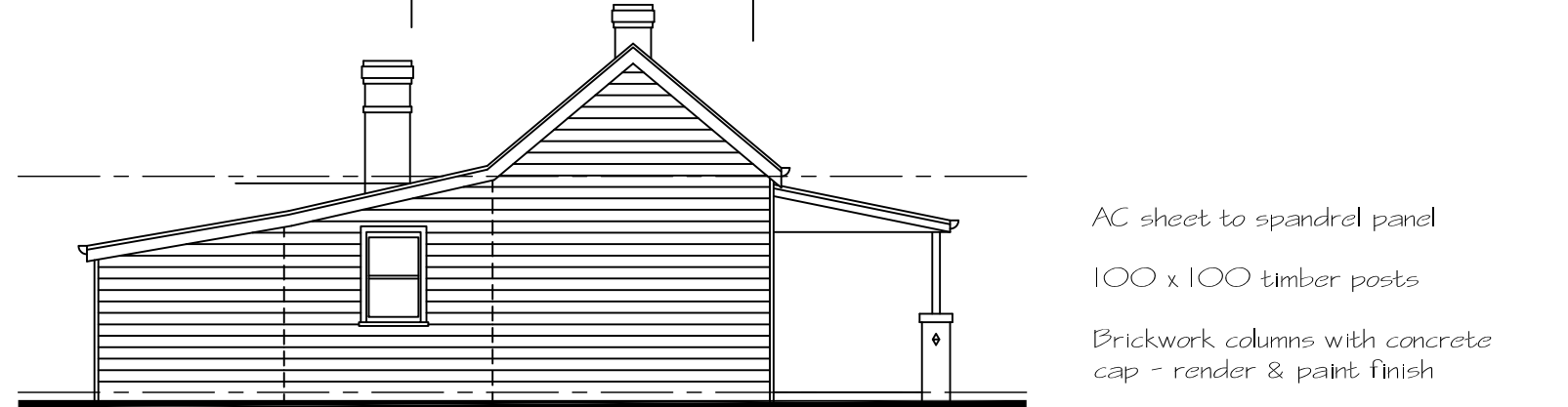
east elevation
